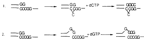
Figure 16. Transient dislocation mechanism.
